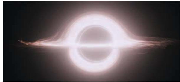
Fig. 2. Gargantua and a variant of the accretion disk seen in Interstellar . Figure created by the Double Negative team using Double Negative Gravitational Renderer, © Warner Bros. Entertainment Inc. (s15). (Used under the terms of the Creative Commons Attribution-NonCommercial-NoDerivs 3.0 (CC BY-NC-ND 3.0) license.)
