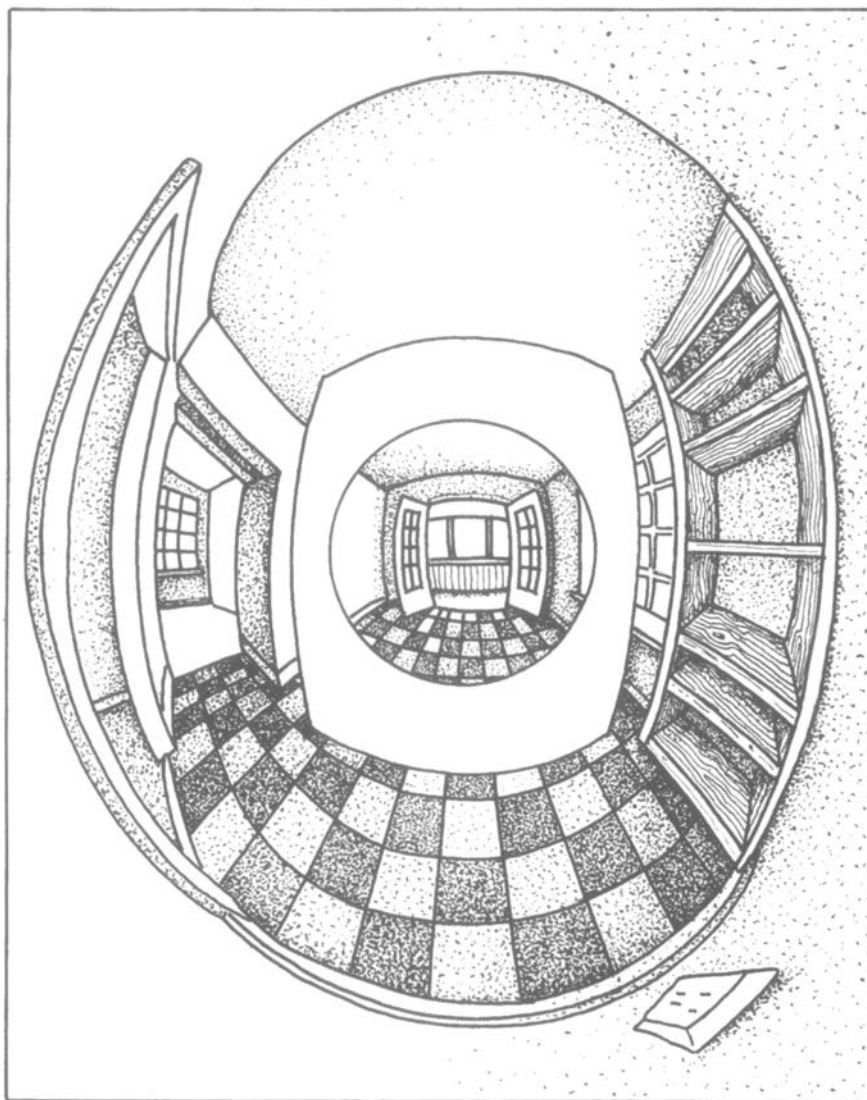
Fig. 6. A sheet of paper traverses the spherical visual field of an ideal observer. When the sheet of paper is outside the sphere, it projects a complete image of its surface onto the spherical field. As portions of the paper enter the sphere, these portions disappear from the spherical image. These portions are circular sections that, starting with a minuscule point, increase in size as the sheet moves into the sphere.
