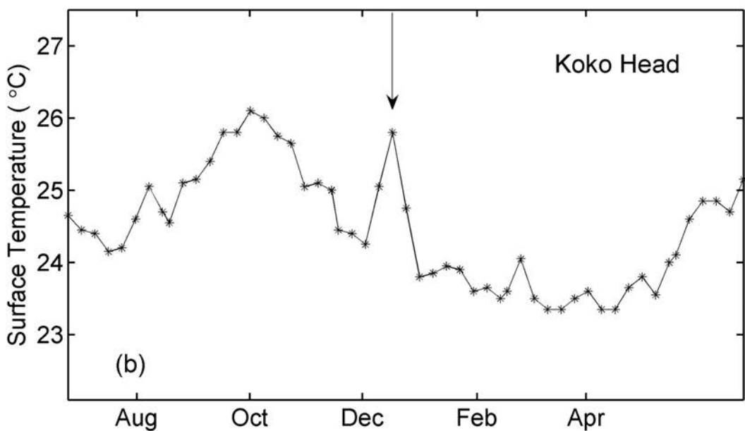
FIGURE 10. The original weekly sea-surface temperature data plotted during the period of the 1976–1977 regime shift at Scripps Pier ( a ) and at Koko Head ( b ). The vertical arrows correspond to change points in the corresponding cumulative sums shown in Figures 4 and 6. The changes in sea-surface temperature indicated by the arrows show that in some cases indications of these events can be observed in the original data.
