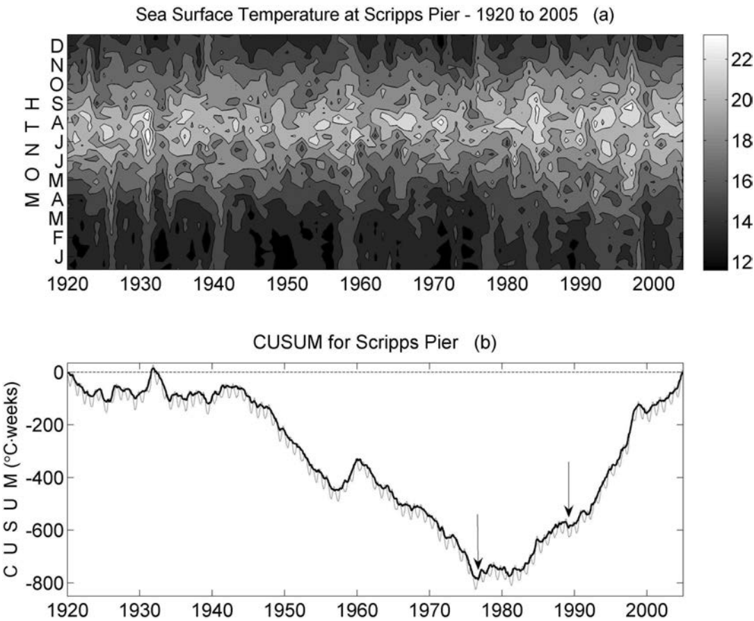
FIGURE 2. The upper panel (a) shows a two-way layout of weekly sea-surface temperature at Scripps Pier, by month, along the y-axis and, by year, along the x-axis. The period extends from 1 January 1920 through 31 December 2004. The warmest temperatures occurred between June and September. The lightest areas correspond in most cases to El Niño warming episodes. The lower panel (b) shows a cumulative sum (CUSUM) of the data shown in (a). The lighter trace shows the cumulative sum based on the original data, and the darker trace shows the cumulative sum with the mean annual cycle removed. In both cases, the global means were removed before the cumulative sums were calculated. The vertical arrows identify regime shifts that occurred during 1976–1977 and 1988–1989.
