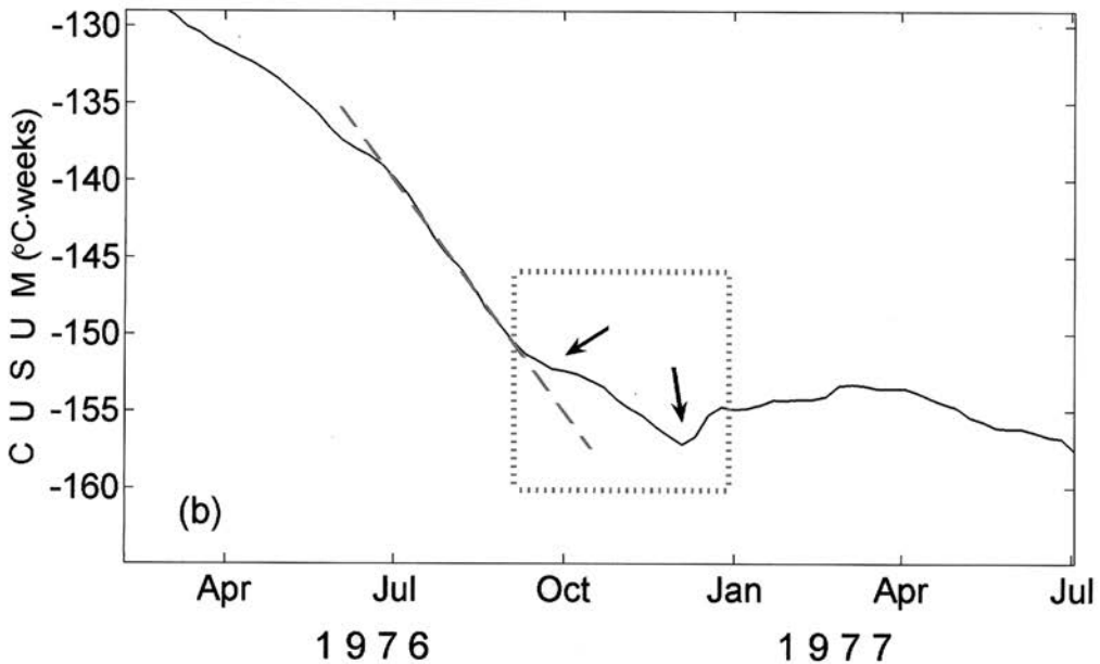
FIGURE 4. The upper panel (a) shows the cumulative sum (CUSUM) at Scripps Pier for the period from early 1976 through 1977. The change points (indicated by dark arrows) within the dark, dashed lines identify the transition period associated with the 1976–1977 regime shift. The gray, dashed box shows the period for the same event at Koko Head, Hawai'i. The lower panel (b) shows the cumulative sum at Koko Head for the period from early 1976 through mid-1977. The gray, dashed box shows the cumulative sum pattern associated with the 1976–1977 event. The dark arrows indicate the turning points that locate the approximate beginning and end of this event. The thin, gray, dashed line shows the slope of the cumulative sum just before the event. In Figure 6a, this event is shown with the slope removed.
