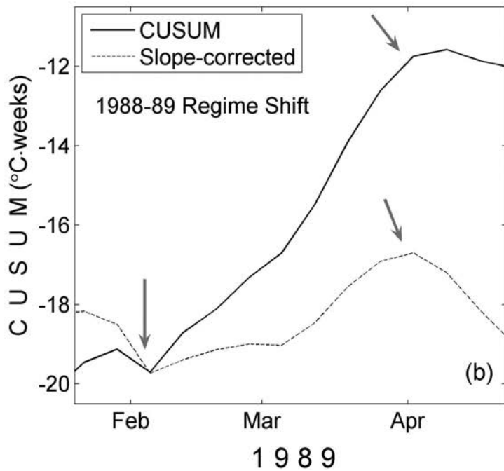
FIGURE 6. The original (solid lines) and slope-corrected (dashed lines) cumulative sums (CUSUM) are shown for the 1976–1977 regime shift at Koko Head in (a), and for the 1988–1989 regime shift at Koko Head in (b). Gray arrows indicate the major turning points that help to delimit these events. See text for details.
