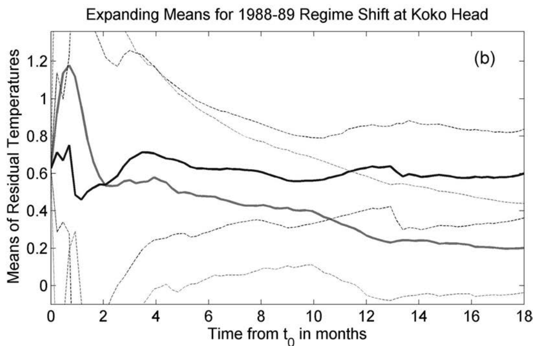
FIGURE 9. Expanding mean temperatures are shown in the forward (gray) and reverse (black) directions starting at the time of the 1988–1989 regime shift for Scripps Pier (a) and Koko Head (b). The dashed lines correspond to the standard error of the mean and thus provide a measure of uncertainty in the mean values that are calculated. Differences in the means before and after the event provide an indication of how well the changes due to this regime shift are sustained and, thus, an indication of its overall impact. See text for details.
